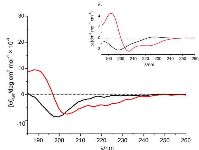
Figure 2. The CD spectrum of peptide 2 (KKWKMRNRNQFWIKIQR-NH 2 ) in water (black line) and in TFE/H 2 O (3:7) (red curve). The CD spectrum of peptide 1 is also shown on the top right side.
