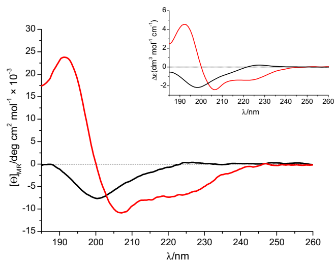
Figure 3. The CD spectrum of peptide 3 (HFRWRQIKIWFQNRMRKWK-NH 2 ) in water (black line) and in TFE/H 2 O (3:7) (red curve).
