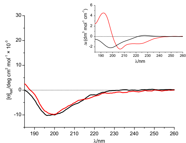
Figure 4. The CD spectrum of peptide 4 (KKWKMRNRNQFWIKIQR-NH 2 ) in water (black line) and in TFE/H 2 O (3:7) (red curve).
