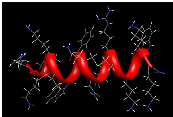
Figure 1. Spatial view of the preferred form ( \alpha -helix structure) for peptide 1 .
